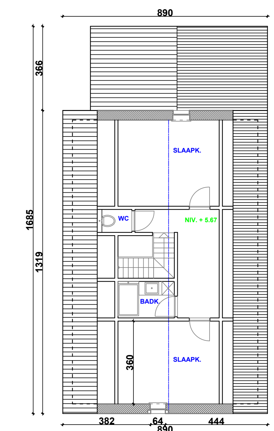
ZOLDER 3
